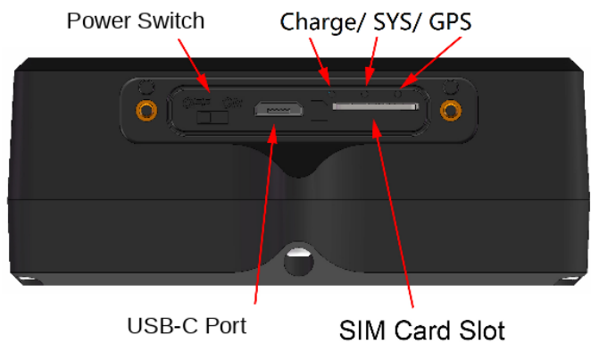
Interfaces (waterproof cover open)
